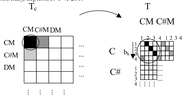
Figure 2: Chord transition matrix for a singles-state HMM [left], transition matrix in the case of a double-states HMM taking into account the position of the chord in the measure [right].
