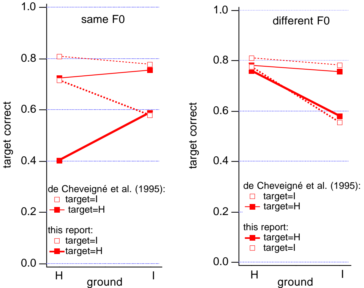
Fig. 8. Identification rate as a function of ground harmonicity for each of the target harmonicity states, at unison and with different F 0 s. Thin lines: (de Cheveigné, et al., 1995), thick lines: this study.
