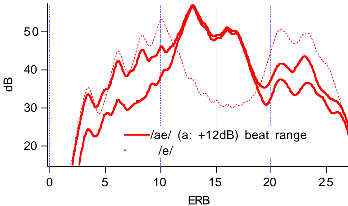
Fig. 4. Excitation patterns for an /ae/ double vowel in which the /a/ is 12 dB more intense than the /e/. The vowels had fundamentals of 124 and 132 Hz respectively. The excitation patterns were derived from an FFT based on a 16 ms Hanning-shaped window, smoothed according to the formulae of (Moore and Glasberg., 1983). The thick curves delimit the range of variation of the excitation pattern for the combined stimulus over its 250 ms duration. The thin dotted curve represents the excitation pattern for /e/ alone.
