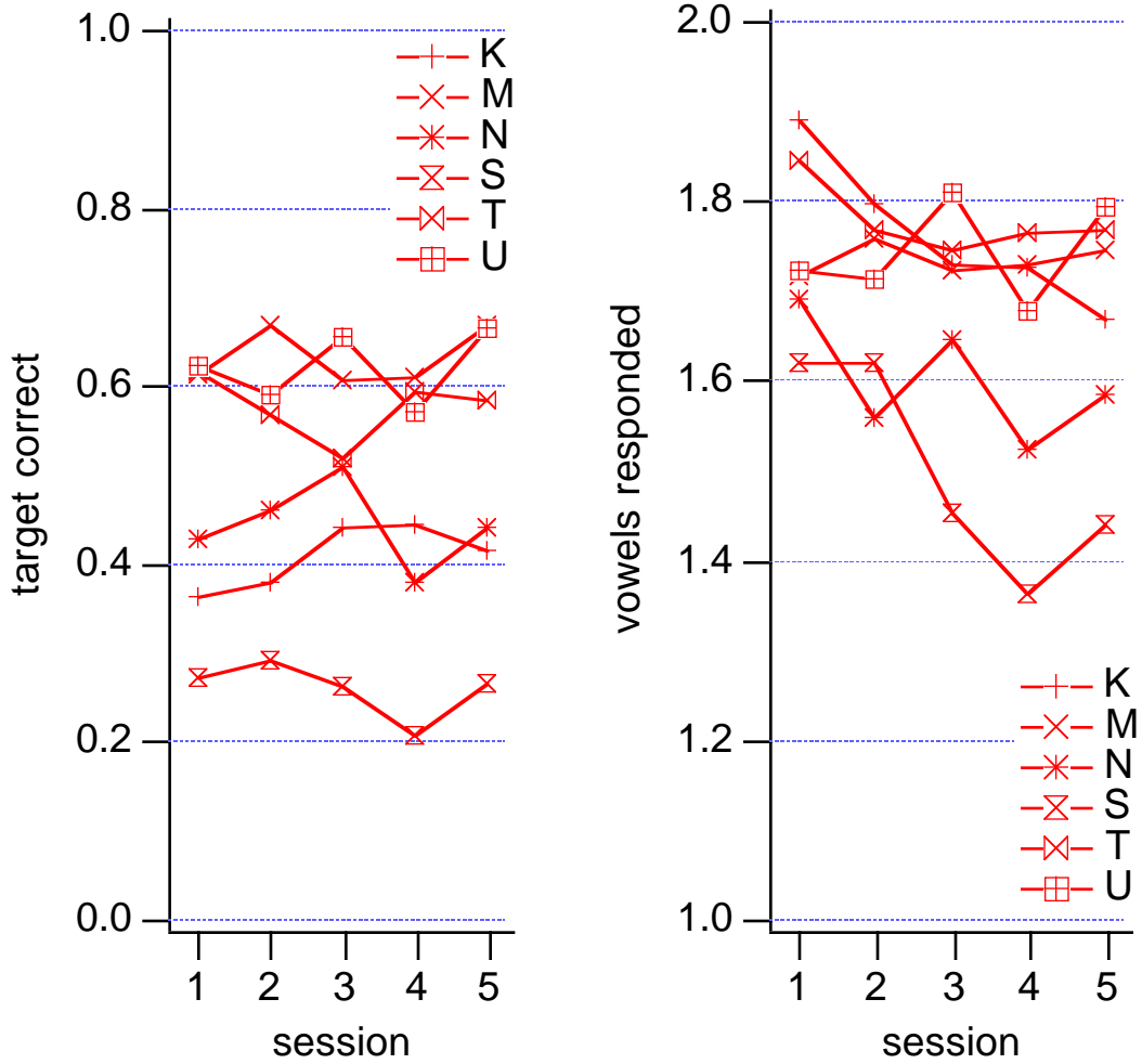
Fig. D-2. Identification rate (left) and number of vowels responded (right) as a function of session number in Experiments 2-4, for all subjects.
